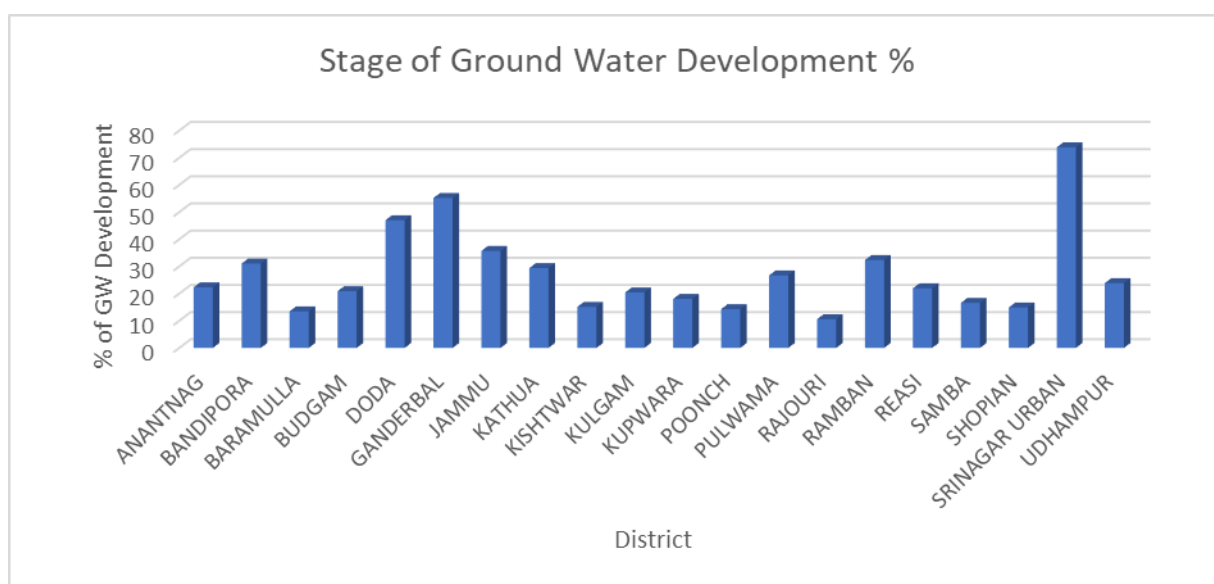
Figure 11 Stage of groundwater Development in %
