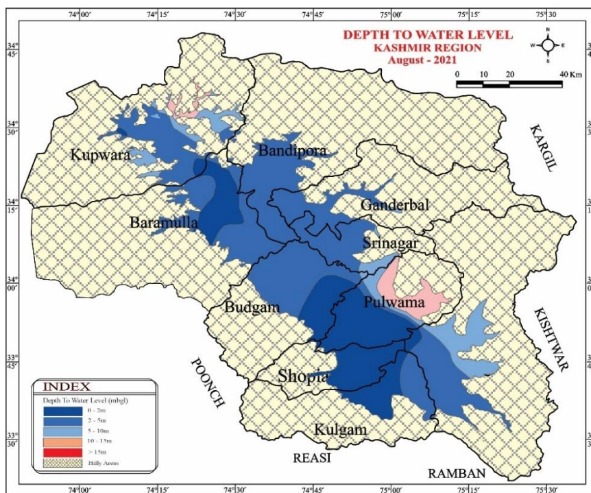
Figure 7 Depth to Water Level, Kashmir Region (August-2021)
