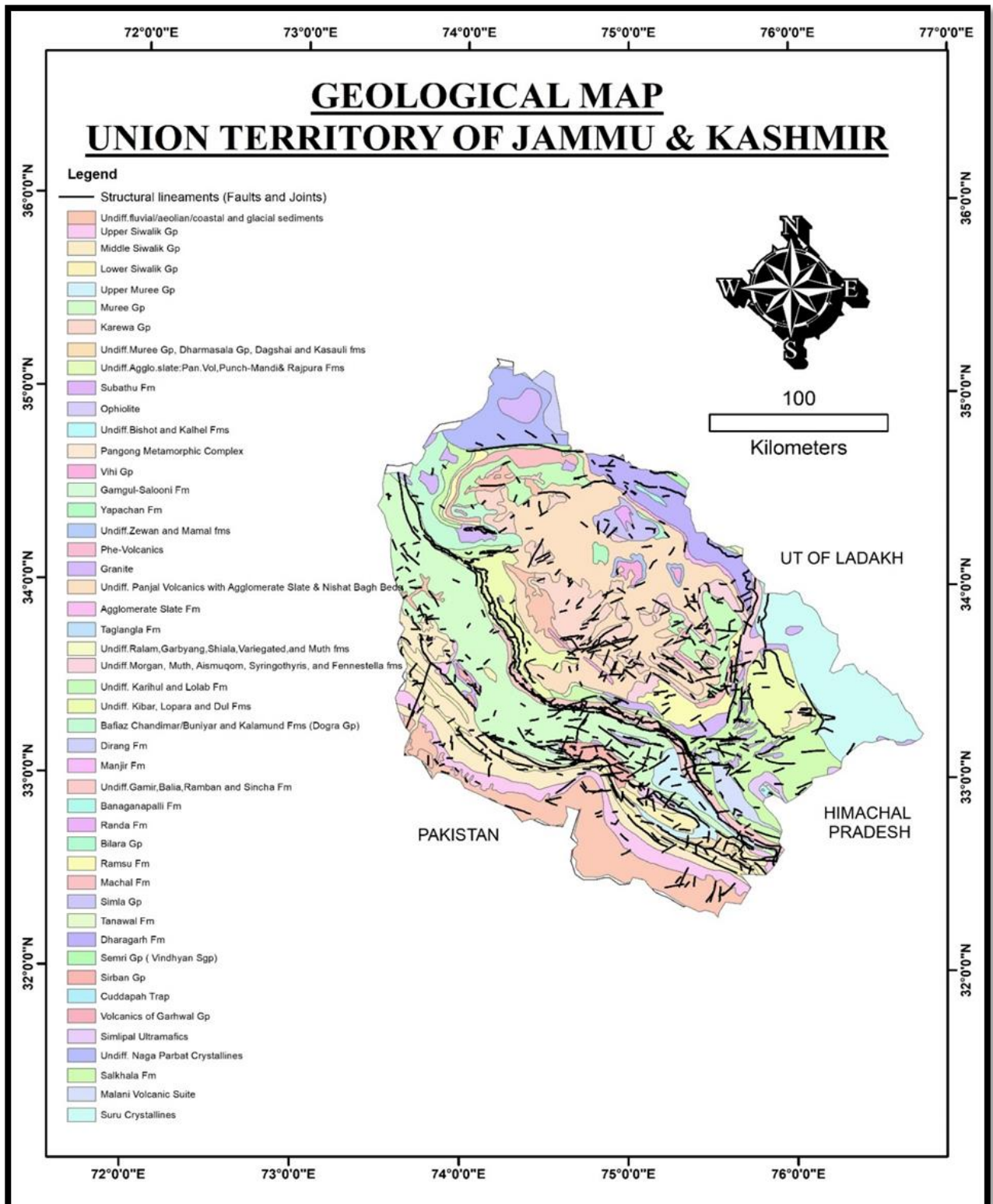
Figure 3 Geological Map of Union Territory of Jammu & Kashmir
