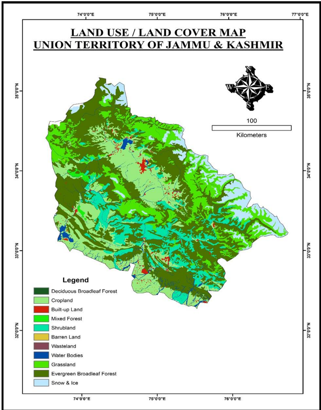
Figure 2 Land Use/land Cover Map of UT of J&K
