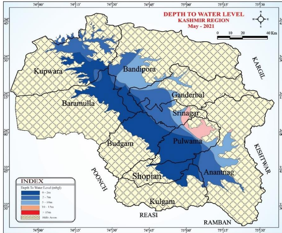
Figure 5 Depth to Water Level, Kashmir Region (May-2021)
