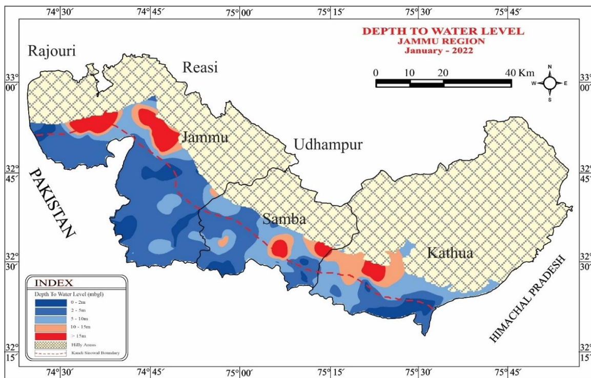
Figure 9 Depth to Water Level, Jammu Region (January-2022)
