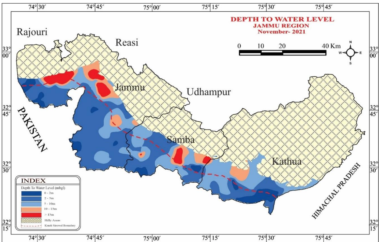
Figure 8 Depth to Water Level, Jammu Region (November-2021)
