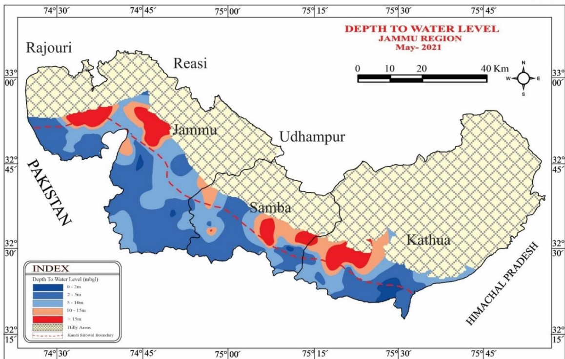
Figure 4 Depth to Water Level, Jammu Region (May-2021)
