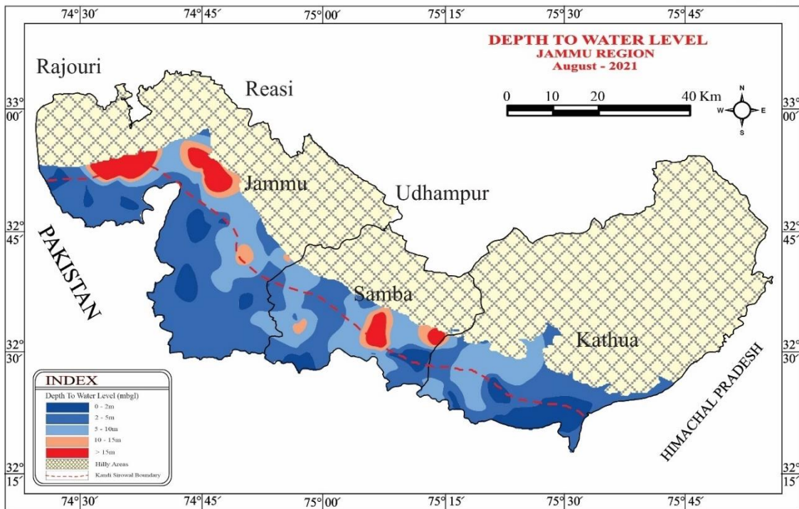
Figure 6 Depth to Water Level, Jammu Region (August-2021)
